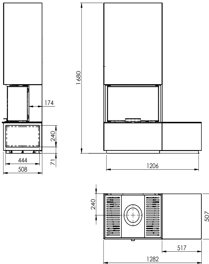
FIG 1c - Monaco Low base + wood shelf / Q-34 UL = mm
